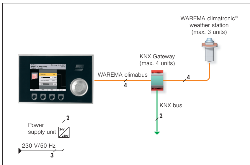
Fig. 2 Overview of a WAREMA climatronic® system as a KNX central control unit
